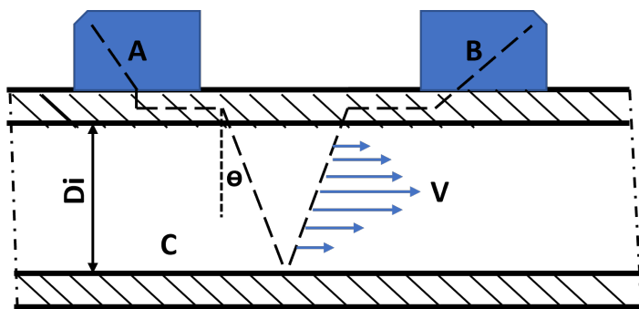
Figure 1: SITRANS FSS200 Sensors mounted in a reflect mode
