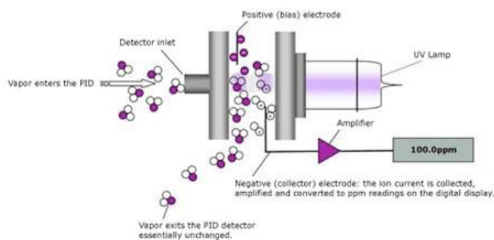
Figure 3: Photoionization Detector
