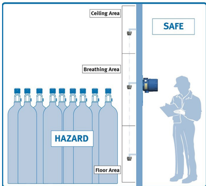
Figure 6: Remote Sensor Placement
