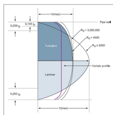
Figure 1: Laminar vs. turbulent flow profiles The laminar profile takes on a parabolic shape where the relationship between the average velocity and centerline velocity is quite dramatic when compared to the turbulent flow profile. Source: Robert Miles, Flow Measurement Engineering Handbook, Velocity profiles related to TD
